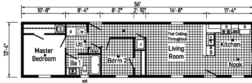
1W1003-P 1456 Approx. 747 Sq. Ft.
